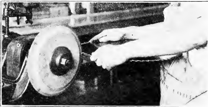
FIG. 178. GUMMING CIRCULAR SAW.
